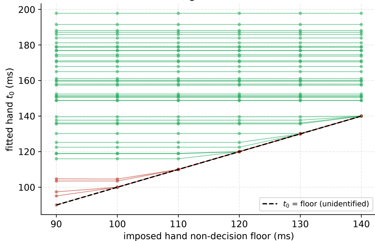
A. HAND t_0 vs imposed floor (43 eligible cells) red = tracks floor; green = stable (identified)
